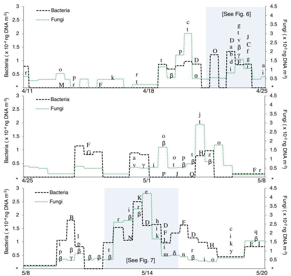
Figure 3 Microbial data from 11 April to 20 May. Values for bacteria and fungi are means of triplicate qPCR runs, time averaged over the sampling interval. Note the difference in scale concentrations between groups. Asterisks represent the lower detection limit of the qPCR assay and letter codes correspond to recovered isolates listed in Tables 3 and 4. Asian, long-range transport events are highlighted with blue boxes
