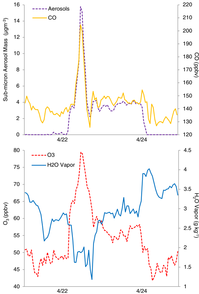
Figure 6 Profile of the 22–23 April long range transport event. Atmospheric data change significantly over the event ( P < 0.05 ) and exhibit free tropospheric signatures (i.e., dry, aerosol/CO/O 3 -enriched
