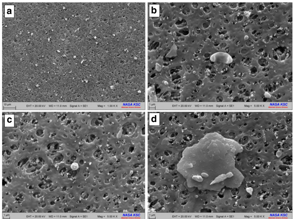
Figure 4 Scanning electron micrographs of PES filters used for capturing airborne microorganisms at the Mt. Bachelor Observatory. a Typical density and distribution of atmospheric particles and microorganisms which appear as bright forms against the darker filter background. b Desiccated, rod-shaped bacterium. c Fungal spore in the center of the micrograph. d Ovoid-shaped bacterial spore attached to a larger particle
