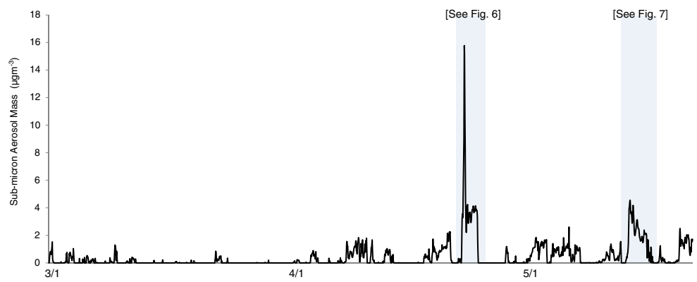
Figure 5 Seasonal dust measured by sub-micron aerosol mass concentration (micrograms per cubic meter). Stormy weather in earlier months kept dust levels low, but values increased towards springtime. Asian, long-range transport events are highlighted with blue boxes
