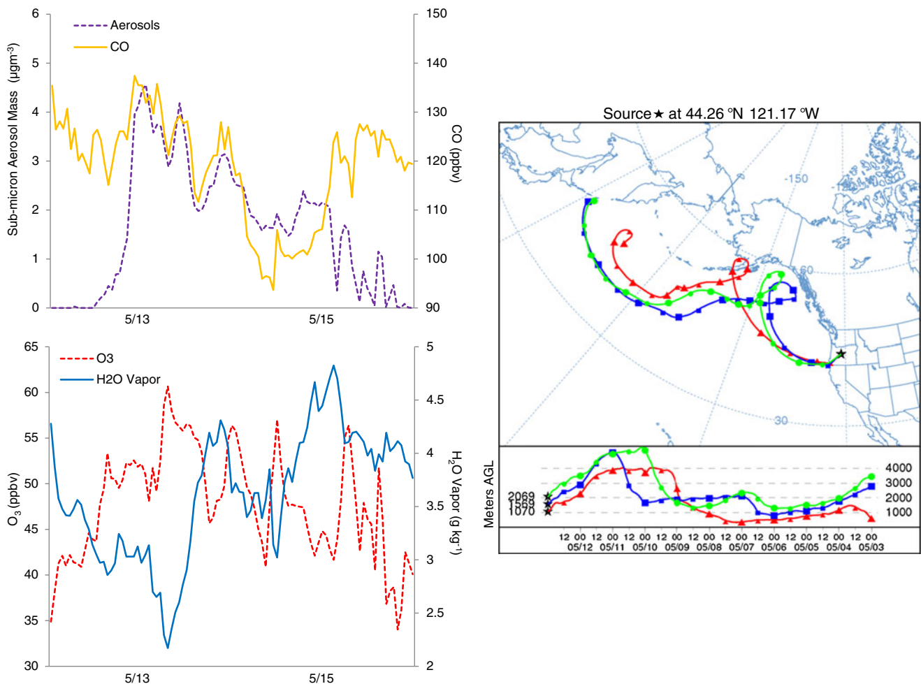
Figure 7 Profile of the 13–15 May long-range transport event. Atmospheric data change significantly over the event ( P < 0.05 ) and exhibit free tropospheric signatures (i.e., dry, aerosol/ \text{CO}/\text{O}_3 -enriched air).
