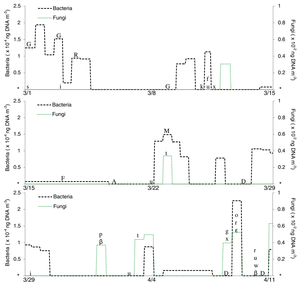
Figure 2 Microbial data from 1 March to 11 April. Values for bacteria and fungi are means of triplicate qPCR runs, time-averaged over the sampling interval. Note the difference in scale concentrations between groups. Asterisks represent the lower detection limit of the qPCR assay and letter codes correspond to recovered isolates listed in Tables 3 and 4
