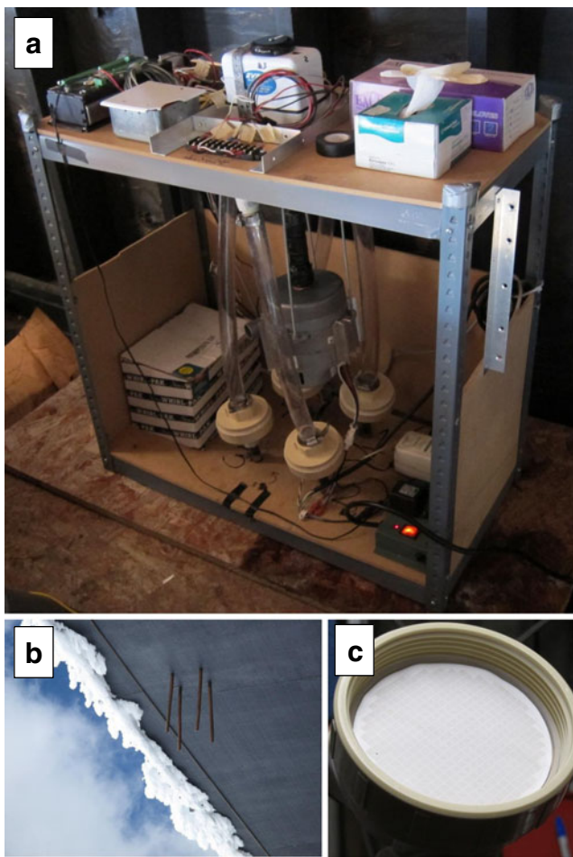
Figure 1 Air sampling apparatus at the Mt. Bachelor Observatory. a A high-vacuum pump, electronics board and four separate filter housings were connected to intake pipes through holes at the base of the device. b Copper intake pipes emerged outside the building, facing into prevailing winds. c Polyethersulfone filter membrane (254 cm 2 , 0.8- \mu m pores) inside plastic housing after an air sampling period
